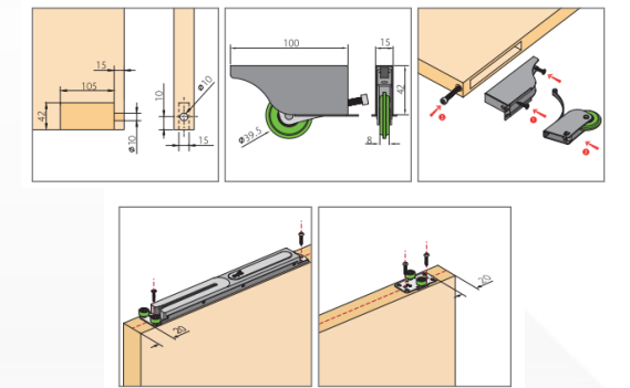
Bottom Rolling Sliding System
