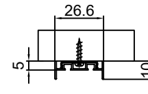
Installation with clasp for track
