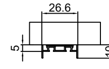
Installation with double-side tape
