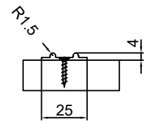
Installation with screw
