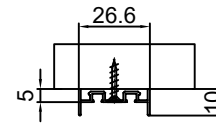
Installation with screw
